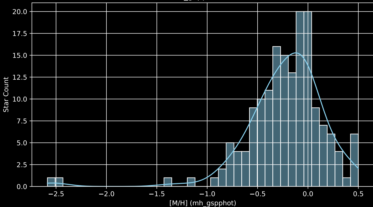
APOGEE DR17 Field: [177+24_MGA [M/H] (mh_gspphot) (n= 167)
