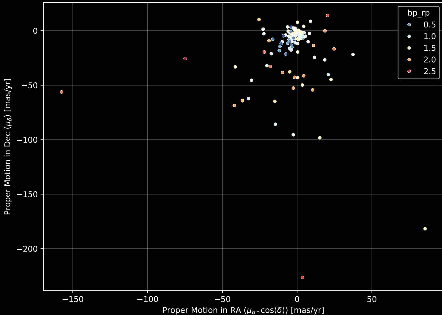
APOGEE DR17 Field: [177+24_MGA] Proper Motion Diagram (n= 169)
