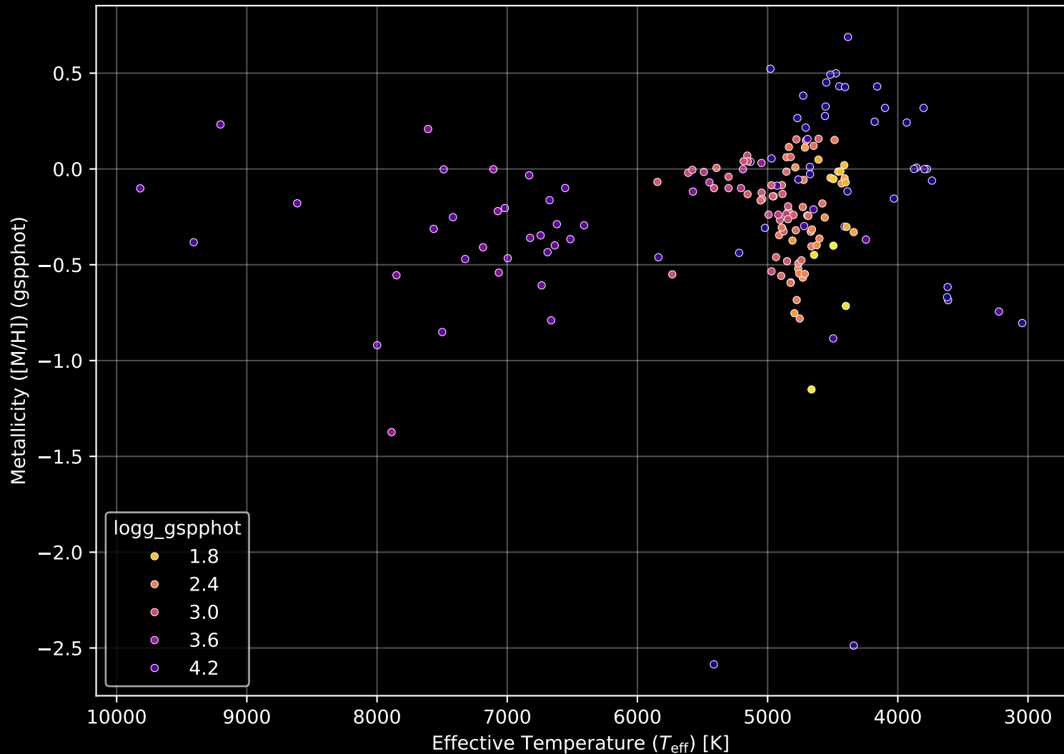
APOGEE DR17 Field: [177+24_MGA] Stellar Population Parameters (n= 169)
