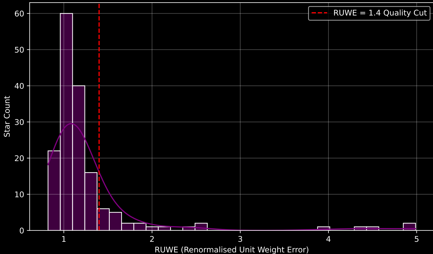
GAPOGEE DR17 Field [177+24_MGA] RUWE Distribution (n= 163)
