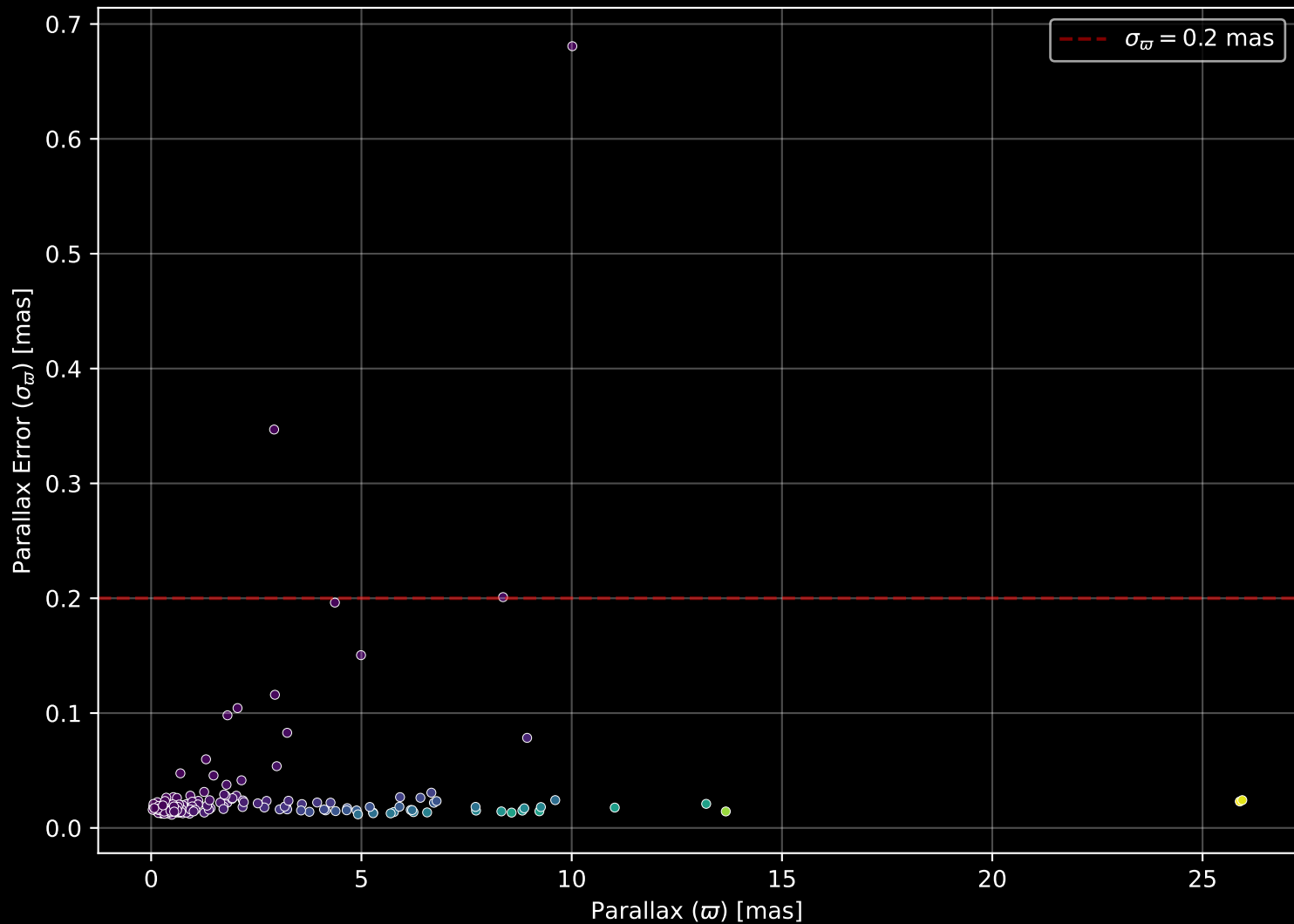
APOGEE DR17 Field: [177+24_MGA] Parallax Quality (n= 169)
