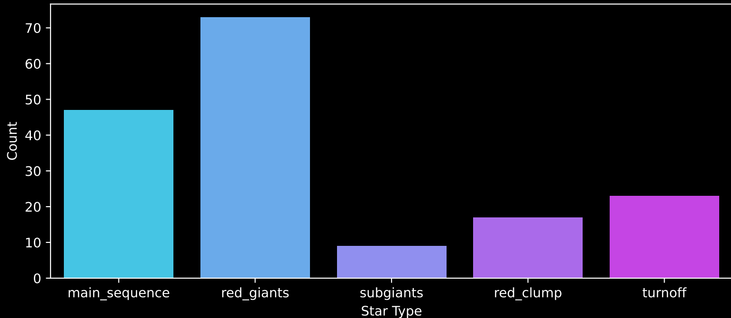
APOGEE DR17 Field: [177+24_MGA] Count plot of Star Type
